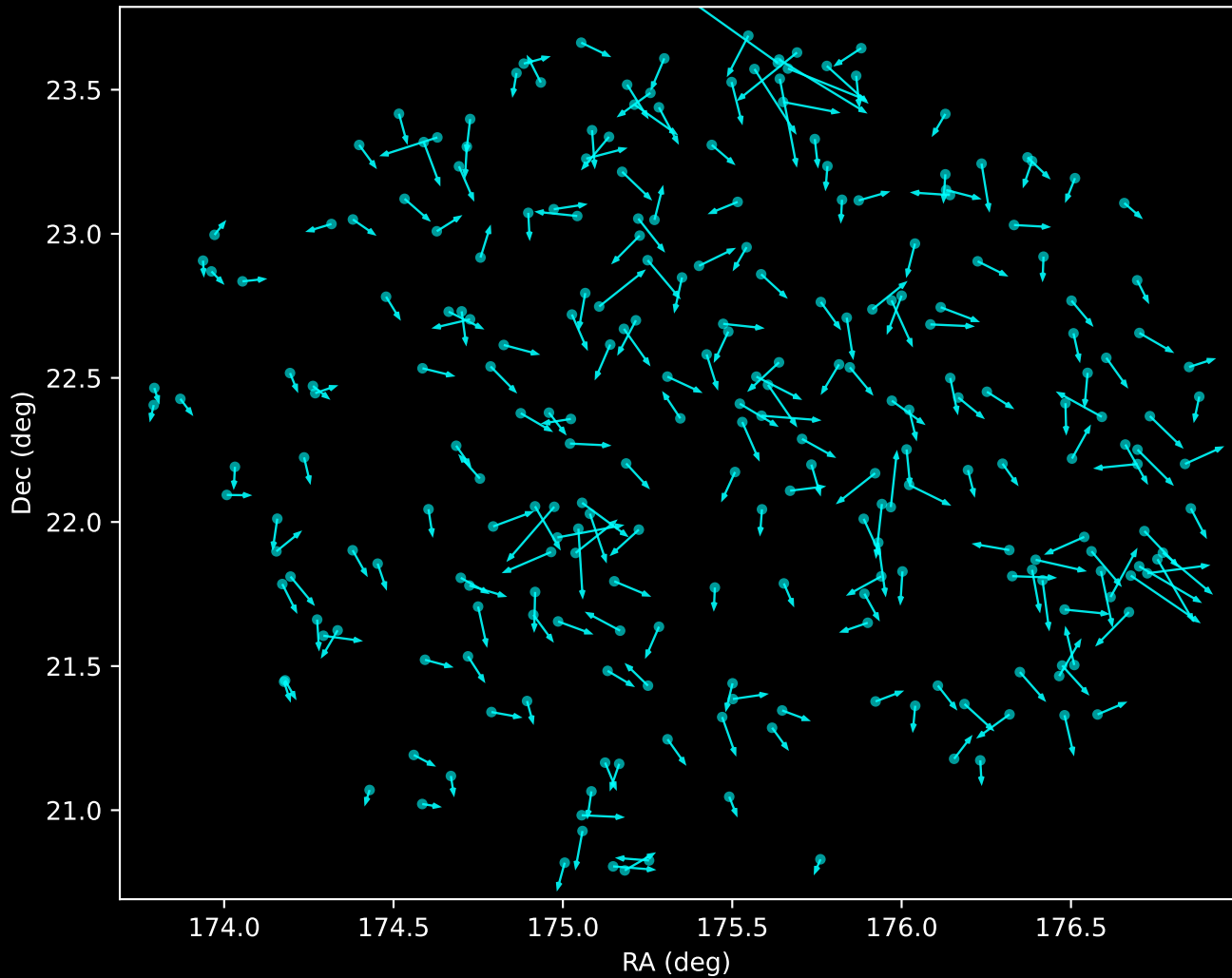
APOGEE DR17 Noise Stream Proper Motion Vectors (n=250)
