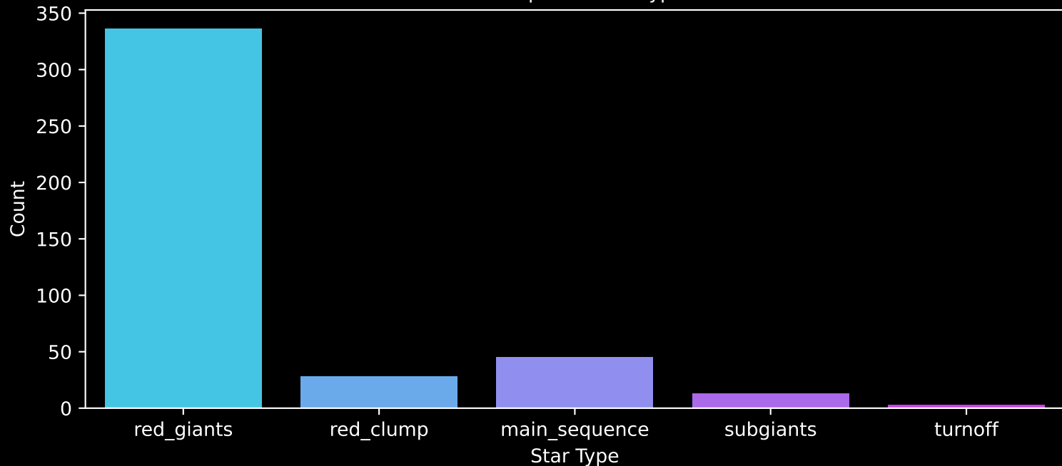
APOGEE DR17 Field: [180-12] Count plot of Star Type
