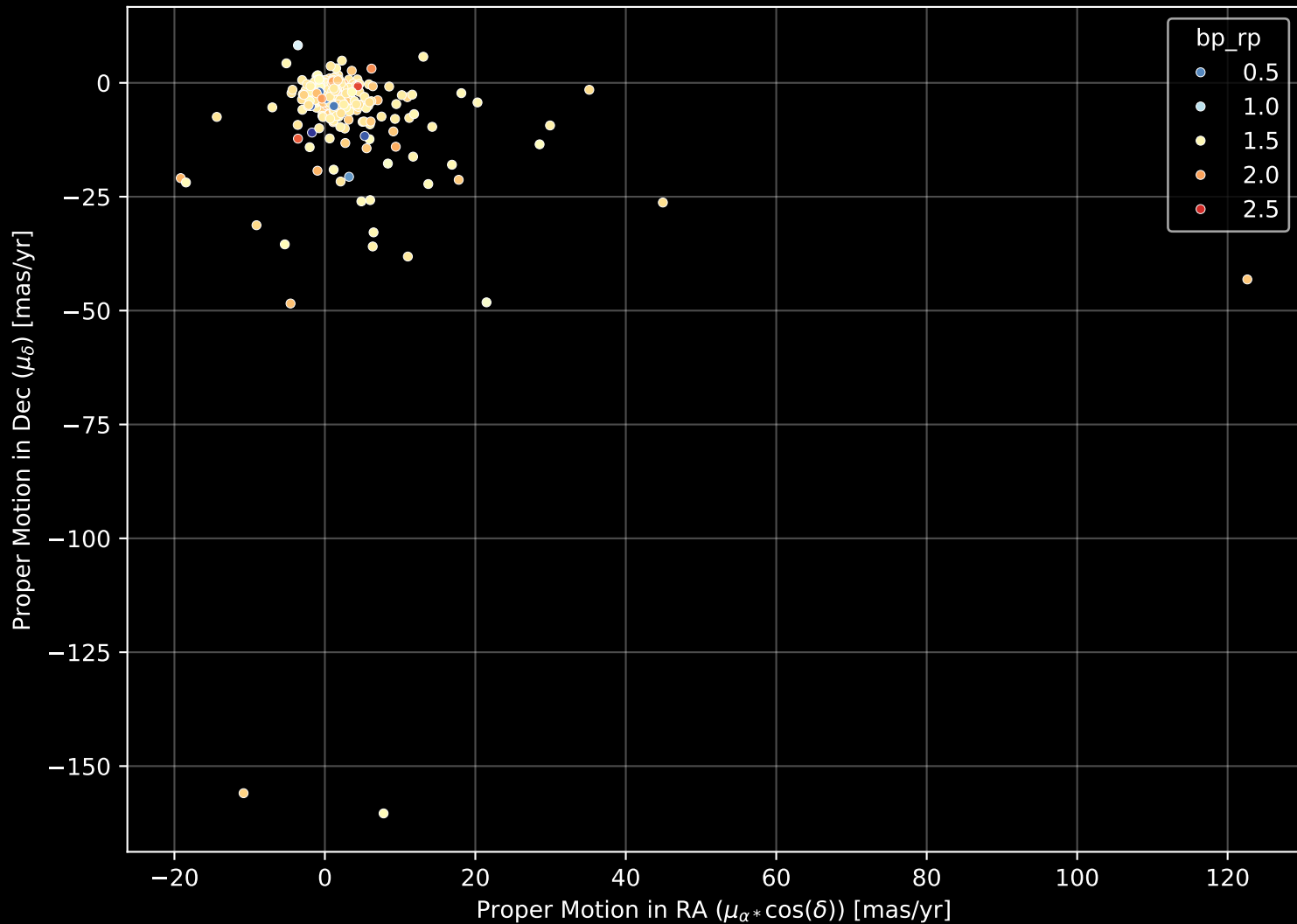
APOGEE DR17 Field: [180-12] Proper Motion Diagram (n= 425)
