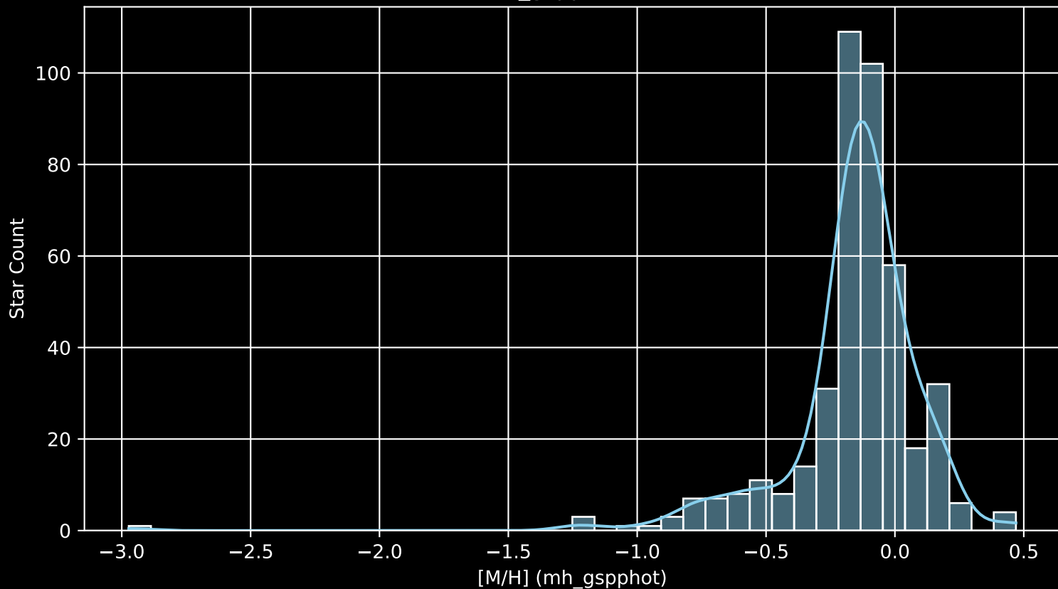
APOGEE DR17 Field: [180-12 [M/H] (mh_gspphot) (n= 424)
