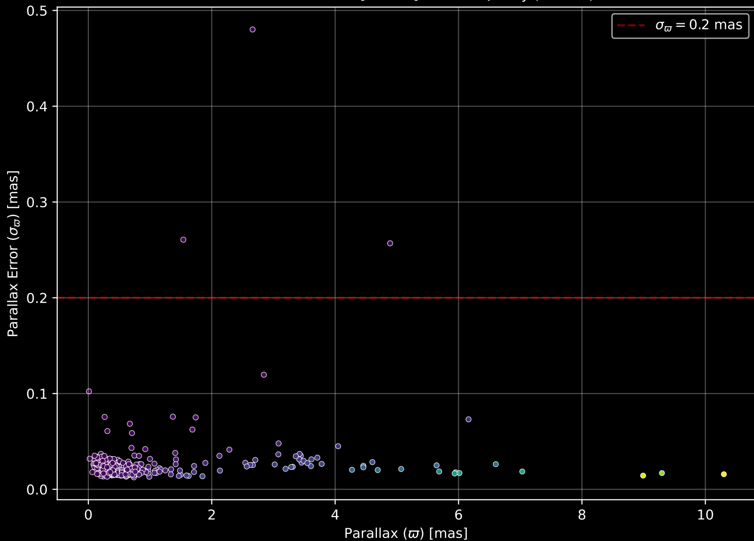
APOGEE DR17 Field: [180-12] Parallax Quality (n= 425)
