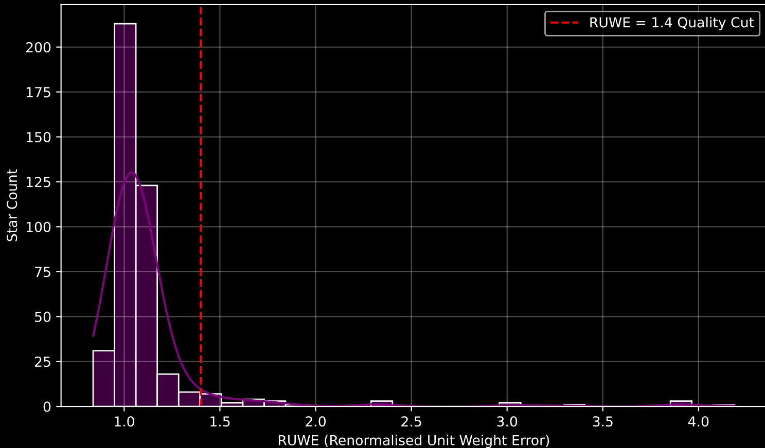
GAPOGEE DR17 Field [180-12] RUWE Distribution (n= 420)
