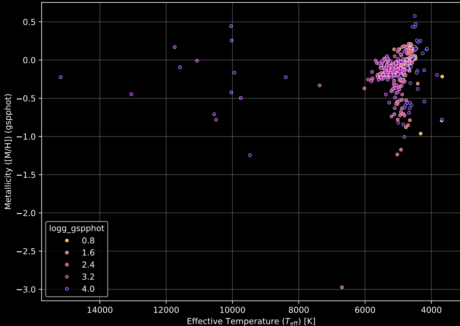
APOGEE DR17 Field: [180-12] Stellar Population Parameters (n= 425)
